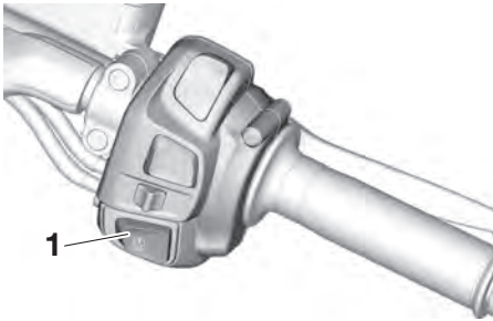
1. "ON" switch
